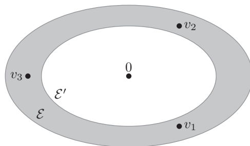
FIG. 4.1. The ellipsoids shown are \mathcal{E} = \mathcal{E}_1(v_1, v_2, v_3) and \mathcal{E}' = \mathcal{E}_{1/2}(v_1, v_2, v_3) . There is an ellipsoid passing through v_1, v_2 , and v_3 because the points are sandwiched between \mathcal{E} and \mathcal{E}' .
