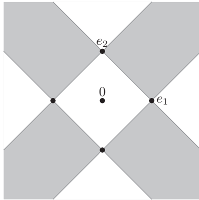
(a) The shaded set is R , those points w for which we can fit an ellipsoid through w and the standard basis vectors.
