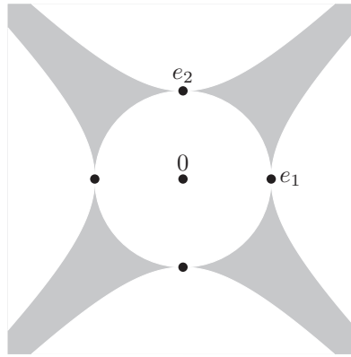
(b) The shaded set is R' , those points w such that w, e_1 , and e_2 satisfy the condition of Corollary 4.4.
