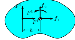
FIGURE 4. Positions for application of forces on a planar rigid body after simplifying assumptions
