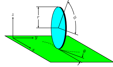
FIGURE 5. The rolling disk
