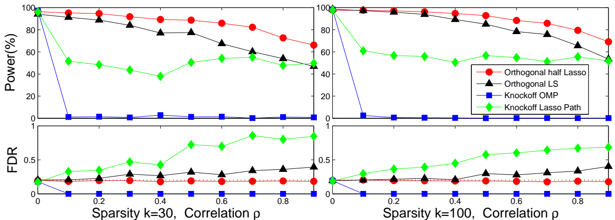
Figure 6: Comparing the orthogonal pseudo knockoff filter with the half Lasso and least squares statistics with the knockoff filter with the OMP and the Lasso path statistics at a nominal FDR q = 20\% by varying the correlation \rho . The figures show the mean power and the mean FDR averaged over 200 trials.
