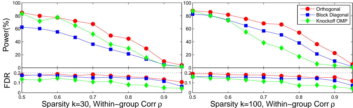
Figure 3: Comparing the orthogonal, the block diagonal pseudo knockoff filter and the knockoff filter with the OMP statistic at nominal FDR q = 20\% by varying the within-group correlation.
