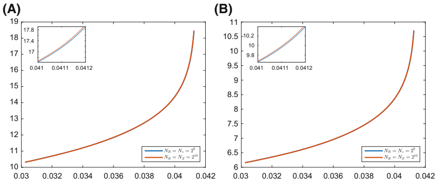
Fig. 1 Resolution study using two meshes. a \log \|\omega_1(t)\|_{L^\infty} . b \log \|u_1(t)\|_{L^\infty}
