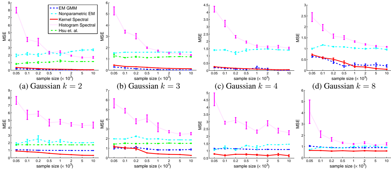
(a) Gaussian k = 2 (b) Gaussian k = 3 (c) Gaussian k = 4 (d) Gaussian k = 8 (e) Gaussian/Gamma k = 2 (f) Gaussian/Gamma k = 3 (g) Gaussian/Gamma k = 4 (h) Gaussian/Gamma k = 8 Figure 3. (a)-(d) Mixture of Gaussian distributions with k = 2, 3, 4, 8 components. (e)-(h) Mixture of Gaussian/Gamma distribution with k = 2, 3, 4, 8 . For the former case, the performances of kernel spectral algorithm converge to those of EM algorithm for mixture of Gaussian model. For the latter case, the performances of kernel spectral algorithm are consistently much better than EM algorithm for mixture of Gaussian model. Spherical Gaussian spectral algorithm does not work for k = 4, 8 since k > l (= 3) causes rank deficiency.
