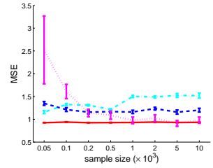
(h) Gaussian/Gamma k = 8
