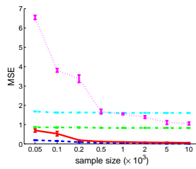
(b) Gaussian k = 3
