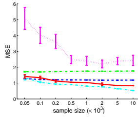
(f) Gaussian/Gamma k = 3
