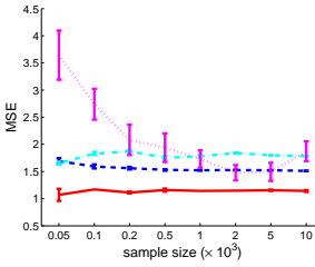
(g) Gaussian/Gamma k = 4
