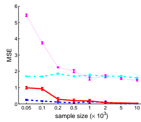
(c) Gaussian k = 4
