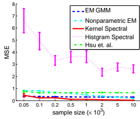
(e) Gaussian/Gamma k = 2
