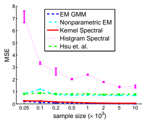
(a) Gaussian k = 2
