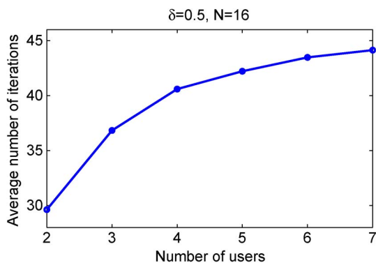
Fig. 9. Average number of iterations versus the number of users Q .
