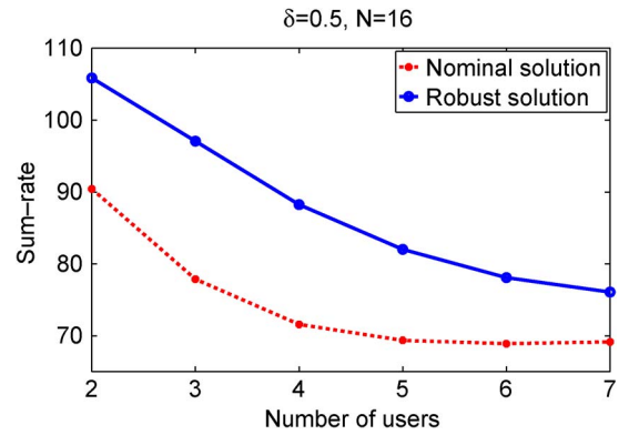
Fig. 4. Sum rate of the system versus the number of users Q .
