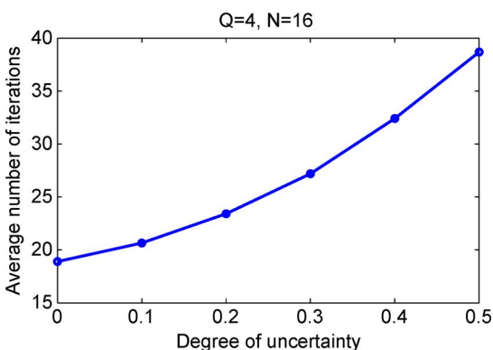
Fig. 8. Average number of iterations versus uncertainty \delta .
