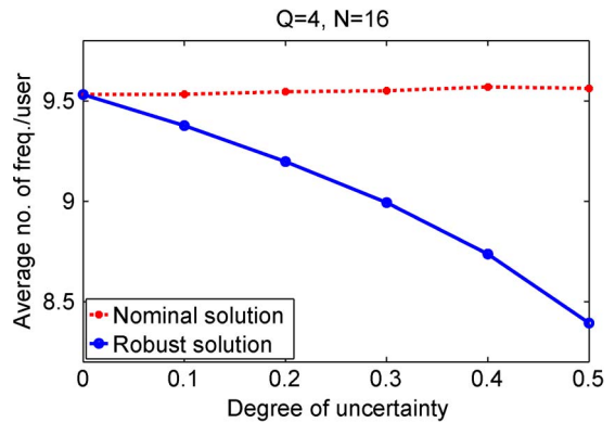
Fig. 6. Average number of channels occupied per user versus uncertainty \delta .
