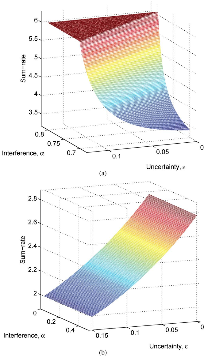
Fig. 2. Simulation results for the antisymmetric system in Fig. 1. Note that the zero uncertainty corresponds to the Nash equilibrium. (a) Sum rate of the system under high interference versus uncertainty and interference. (b) Sum rate of the system under low interference versus uncertainty and interference.
