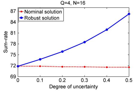
Fig. 3. Sum rate of the system versus uncertainty \delta .
