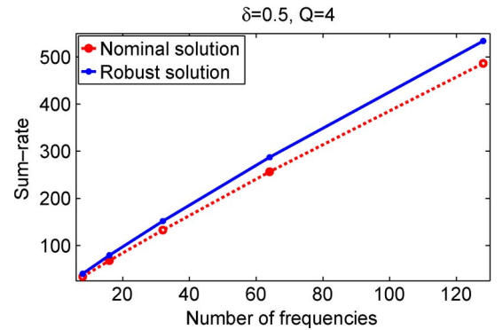
Fig. 5. Sum rate of the system versus the number of frequencies N .
