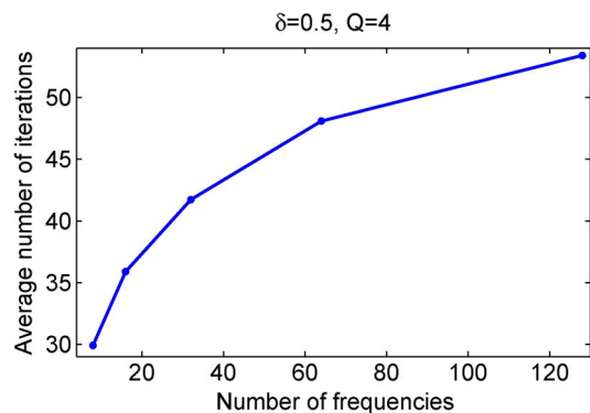
Fig. 10. Average number of iterations versus the number of frequencies N .
