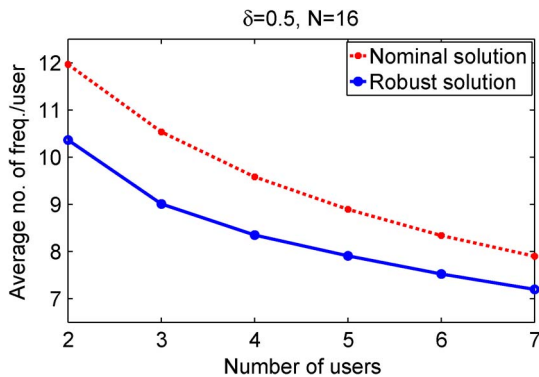
Fig. 7. Average number of channels occupied per user versus the number of users Q .
