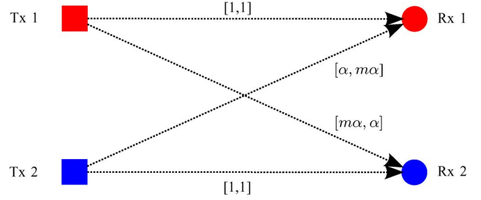
Fig. 1. Antisymmetric system where Q = 2 , N = 2 , \epsilon_1 = \epsilon_2 = \epsilon , and the noise variances for both users in both frequencies is \sigma^2 . The channel gains are |H_{11}(1)|^2 = |H_{11}(2)|^2 = |H_{22}(1)|^2 = |H_{22}(2)|^2 = 1 , |H_{12}(2)|^2 = |H_{21}(1)|^2 = \alpha , and |H_{12}(1)|^2 = |H_{21}(2)|^2 = m\alpha , with m > 1 and 0 < \alpha < 1 . The power allocations for this system at the RE are presented in (23).
