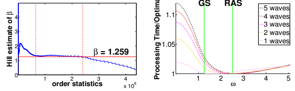
Figure 3: Hill plot of Facebook task durations.
