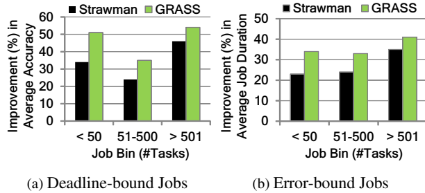
Figure 12: Comparing GRASS’s learning based switching approach to a strawman that approximates two waves of tasks. GRASS is 30% – 40% better than the strawman.
