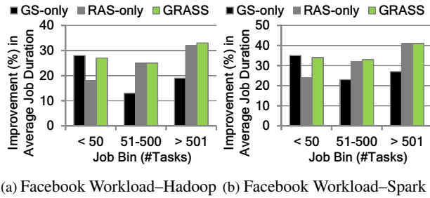
Figure 11: GRASS’s switching is 20% better than using GS or RAS all through for error-bound jobs. We use the Facebook workload and LATE as baseline.
