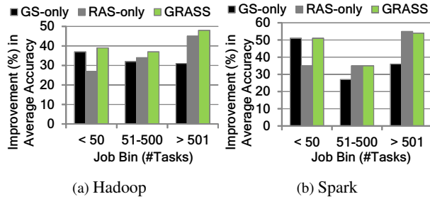
Figure 10: GRASS’s switching is 25% better than using GS or RAS all through for deadline-bound jobs. We use the Facebook workload and LATE as baseline.
