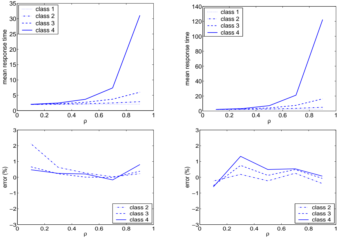
(a) M/M/2 with four classes
