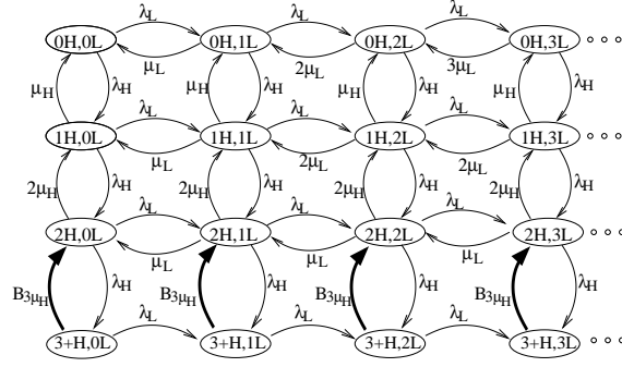
Figure 2: This chain illustrates the case of two priority classes and three servers. The busy period transitions are replaced by a Coxian phase-type distribution matching three moments of the busy period duration, as shown in Figure 1.
