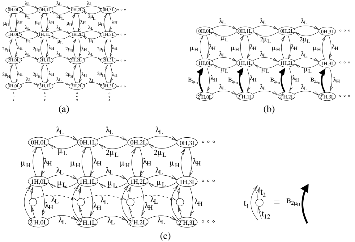
Figure 1: (a) Markov chain for an M/M/2 queue with two priority classes. This Markov chain is infinite in two dimensions. Via the Dimensionality Reduction technique, we arrive at the chain in (b), which uses busy period transitions, and is only infinite in one dimension. In (b), the busy period is represented by a single transition. In (c), the busy period is represented by a two phase PH distribution (with Coxian representation), yielding a 1D-infinite Markov chain.
