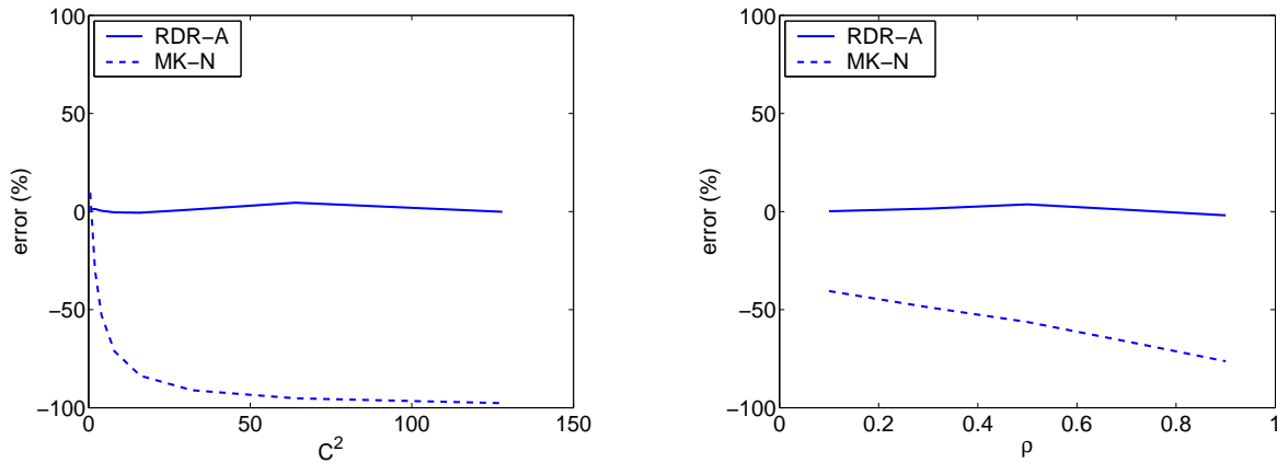
Figure 10: Effect of aggregation. Graphs show error in mean delay of the 4th (lowest priority) class in the MK-N and RDR-A approximations for an M/PH/2 with SMART prioritization, as compared with simulation. On the left as a function of C^2 where \rho = 0.8 , and on the right as a function of \rho where C^2 = 8 . The classes all have a 2-phase PH distribution with the same squared coefficient of variation C^2 and different means: 1, 2, 4, and 8.
