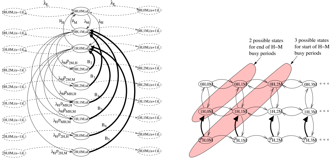
Figure 3: (Left) Portion of the 1D-infinite chain used to compute mean response time for low-priority jobs in the case of three priority classes and two servers, and all exponential service times. (Right) Chain used to compute moments of the durations of the six busy period transitions.
