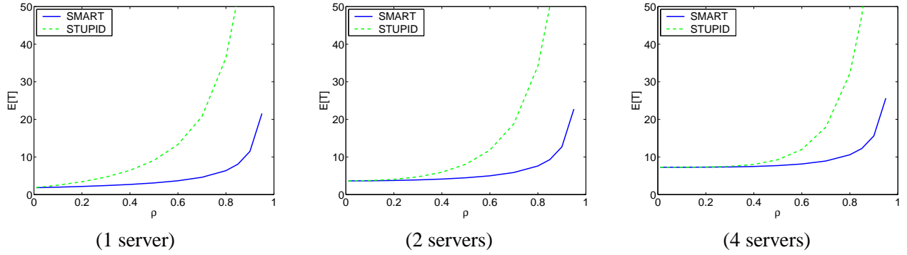
Figure 9: Mean response time under SMART versus STUPID prioritization in a 2-class system, where the classes are exponentially distributed with means one and ten respectively, for the case of one server, two servers, and four servers.
