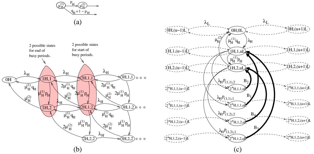
Figure 4: (a) A 2-phase PH distribution with Coxian representation. (b) Markov chain which will be used to compute the high-priority job busy periods, in the case where high-priority job size have a PH distribution with Coxian representation shown in (a). (c) Chain for a system with two servers and two priority classes where high priority jobs have Coxian service times.
