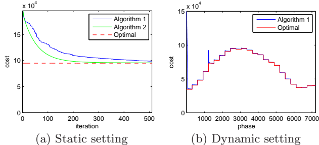
Figure 2: Convergence of Algorithm 1 and 2.
