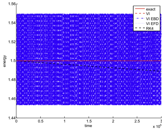
Fig. 5. LC circuit (no resistors) with step size h = 0.05 . Comparison of the exact solution (exact) and the numerical solution using the three different variational integrators, midpoint rule (VI), backward Euler (VI EBD), and forward Euler (VI EFD), a Runge-Kutta method of fourth order (RK4). The long-time energy is (qualitatively) preserved for VI, VI EBD, and VI EFD. The lines of exact and VI lie on top of each other at energy value 1.5. The use of RK4 leads to an artificial energy decay.
