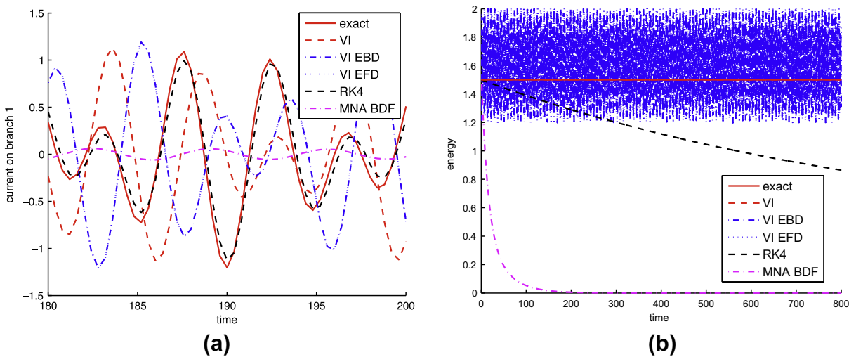
Fig. 4. LC circuit (no resistors) with step size h = 0.4 . Comparison of the exact solution (exact) and the numerical solution using the three different variational integrators, midpoint rule (VI), backward Euler (VI EBD), and forward Euler (VI EFD), a Runge–Kutta method of fourth order (RK4), and a BDF method of second order based on MNA (MNA BDF). (a) The use of variational integrators (VI, VI EBD, VI EFD) leads to a phase shifting in the numerical solution of the current. With the BDF method, the oscillations are damped out. (b) The energy is (qualitatively) preserved for VI, VI EBD, and VI EFD. The lines of exact and VI lie on top of each other at energy level 1.5. The use of RK4 and BDF leads to an artificial energy decay.
